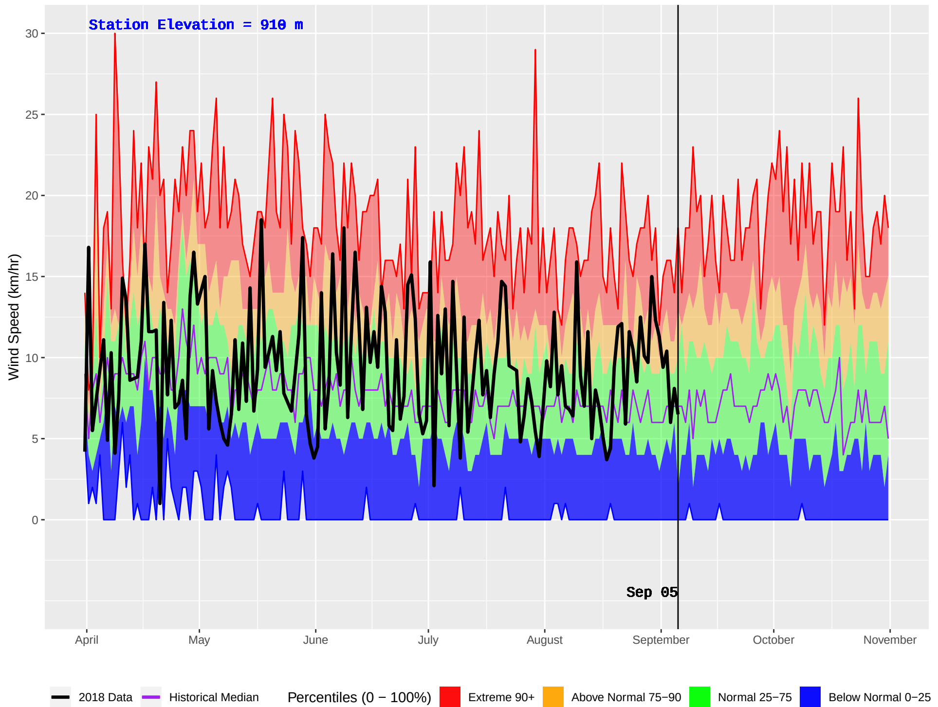
NAZKO (211) : Historical (1981–2016) and Current (2018) Daily Wind Speed
