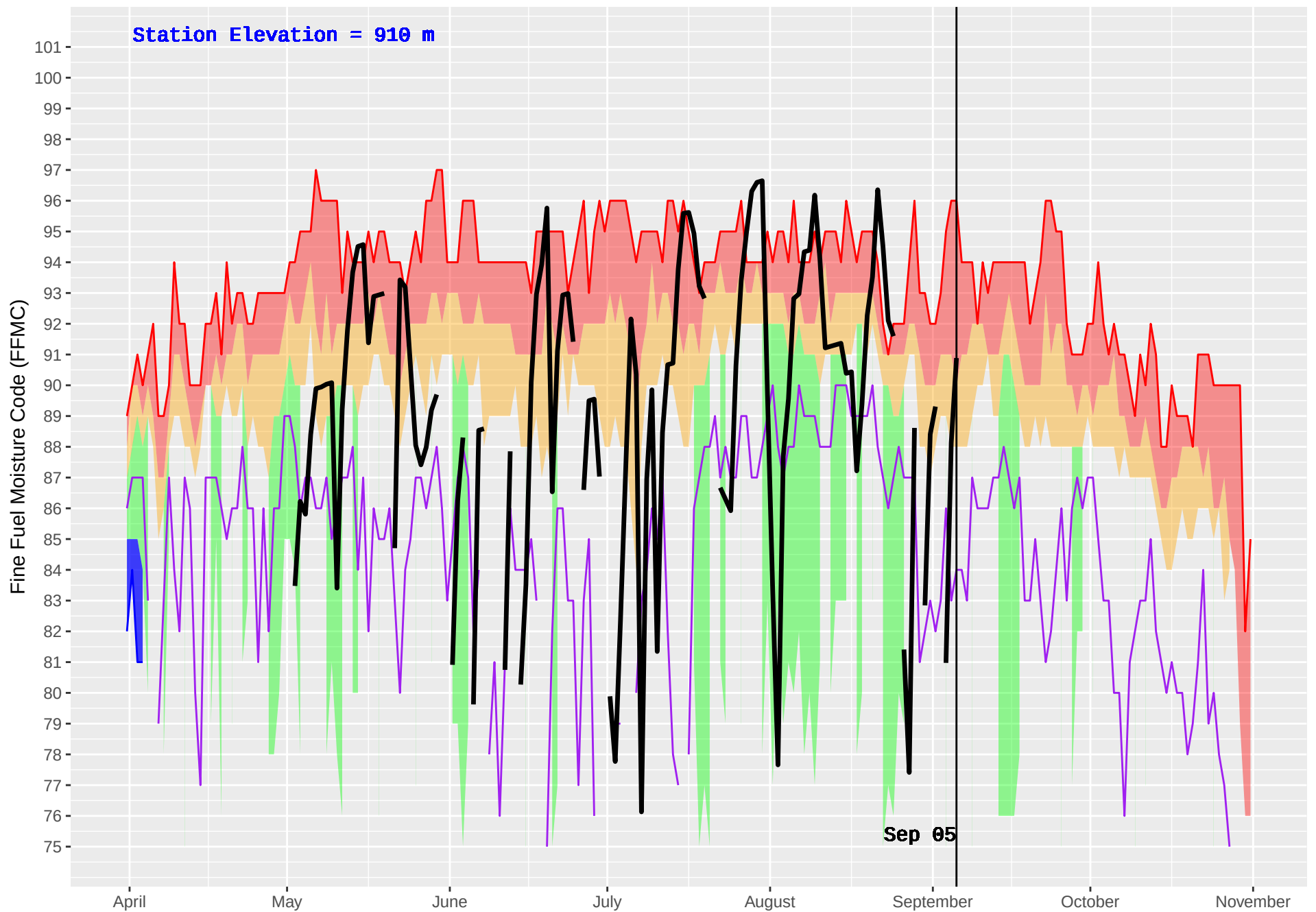
NAZKO (211) : Historical (1981–2016) and Current (2018) Daily Fine Fuel Moisture Code (FFMC)
