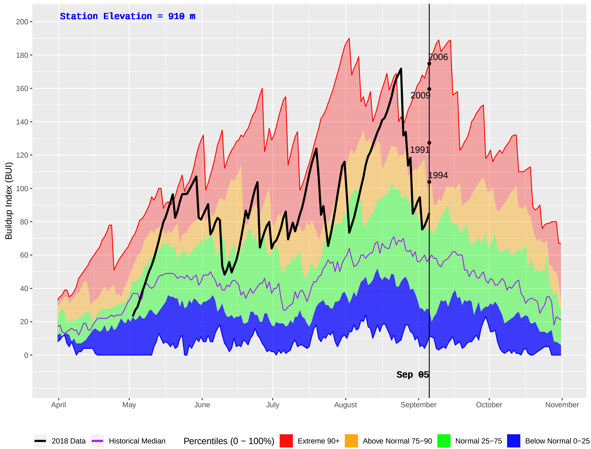
NAZKO (211) : Historical (1981–2016) and Current (2018) Daily Buildup Index (BUI)
